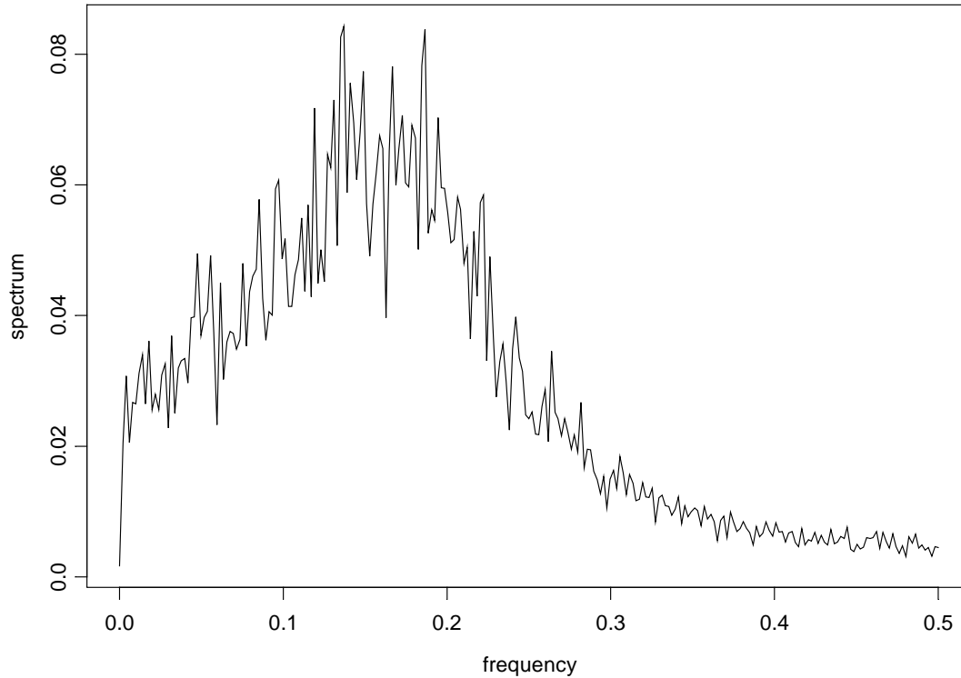
Figure 2. Power spectrum of 500 solutions over 500 steps of the annual output growth in the model, X . N = 100 , \alpha = 1 , \beta = 0.6 , sd_1 = 0.0375 , sd_2 = 0.525 .
